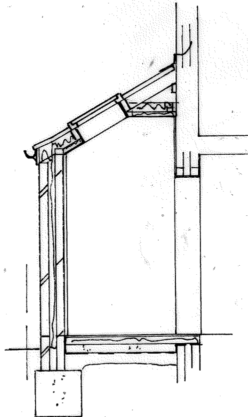
SECTION 1:50
